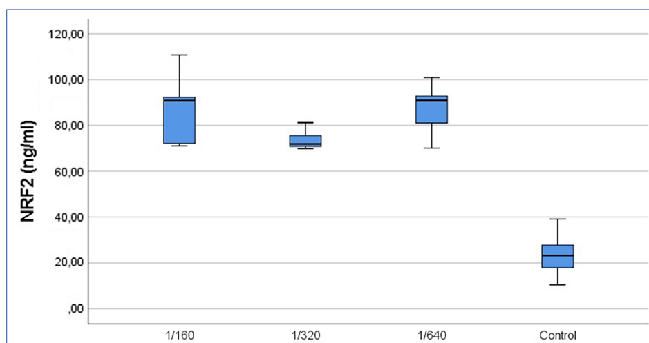
Figure 3. NRF2 levels in the study groups (means +/- standard deviation).
